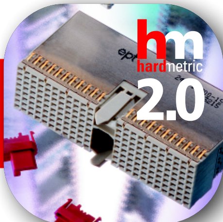
hm 2.0 hardmetric plug-in connector complying with IEC 61076-4-101
